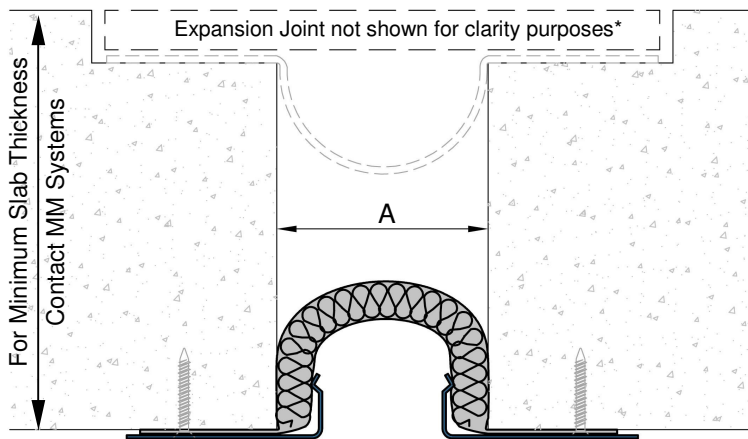
Under Slab Pyro-Flex Series (*elastomeric or metal cover plate required)
