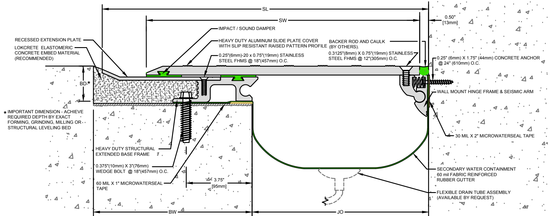
SSP-EHD Series Expansion Joint (Slab-to-Wall)
