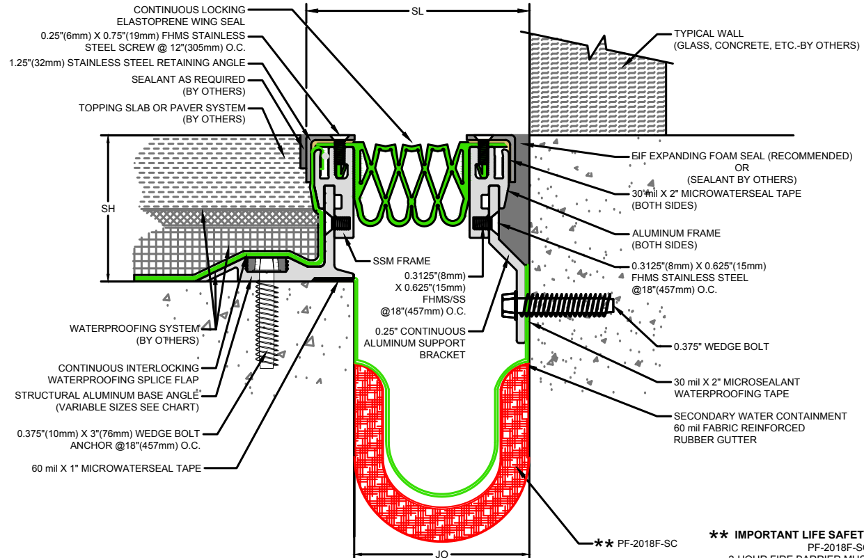
SSM-TM Series Expansion Joint (Slab-to-Throat Mount)
