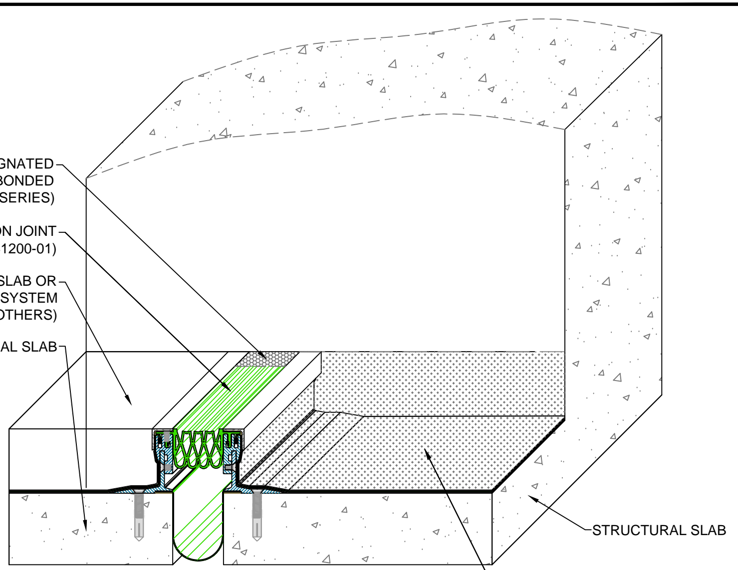
SSM End Termination Expansion Joint (Transition)
