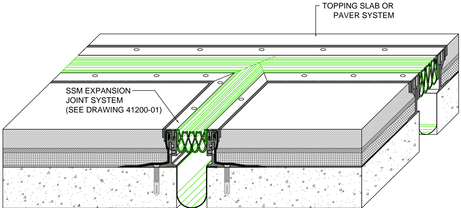
SSM Series Tee Transition Expansion Joint (Slab-to-Slab)
