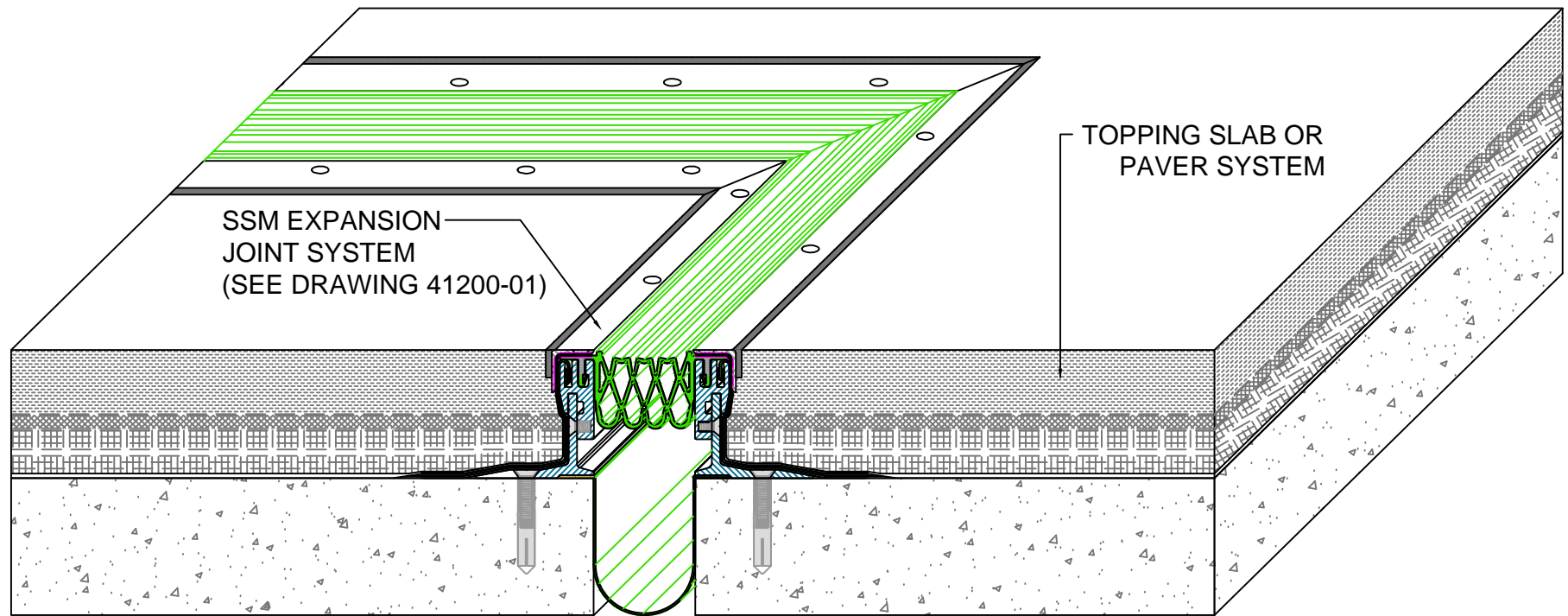
SSM Series 90° Turn Transition Expansion Joint (Slab-to-Slab)
