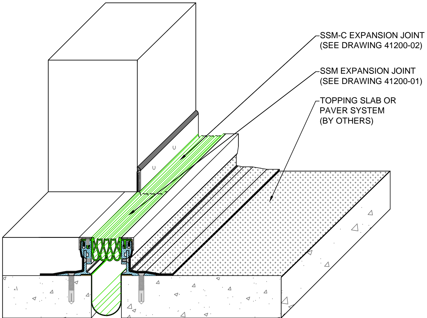
SSM-to-SSM-C Inline Expansion Joint (Inline Transition)
