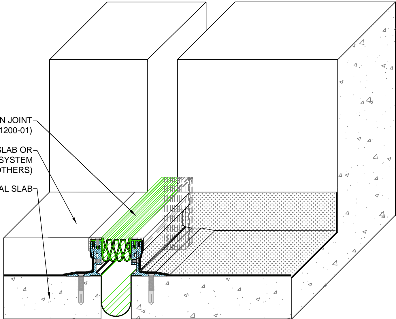
SSM Turn-Down Expansion Joint (Turn-Down Transition)
