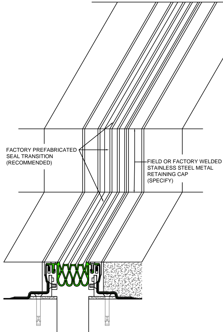
SSM Curb Expansion Joint (Curb Transition)
