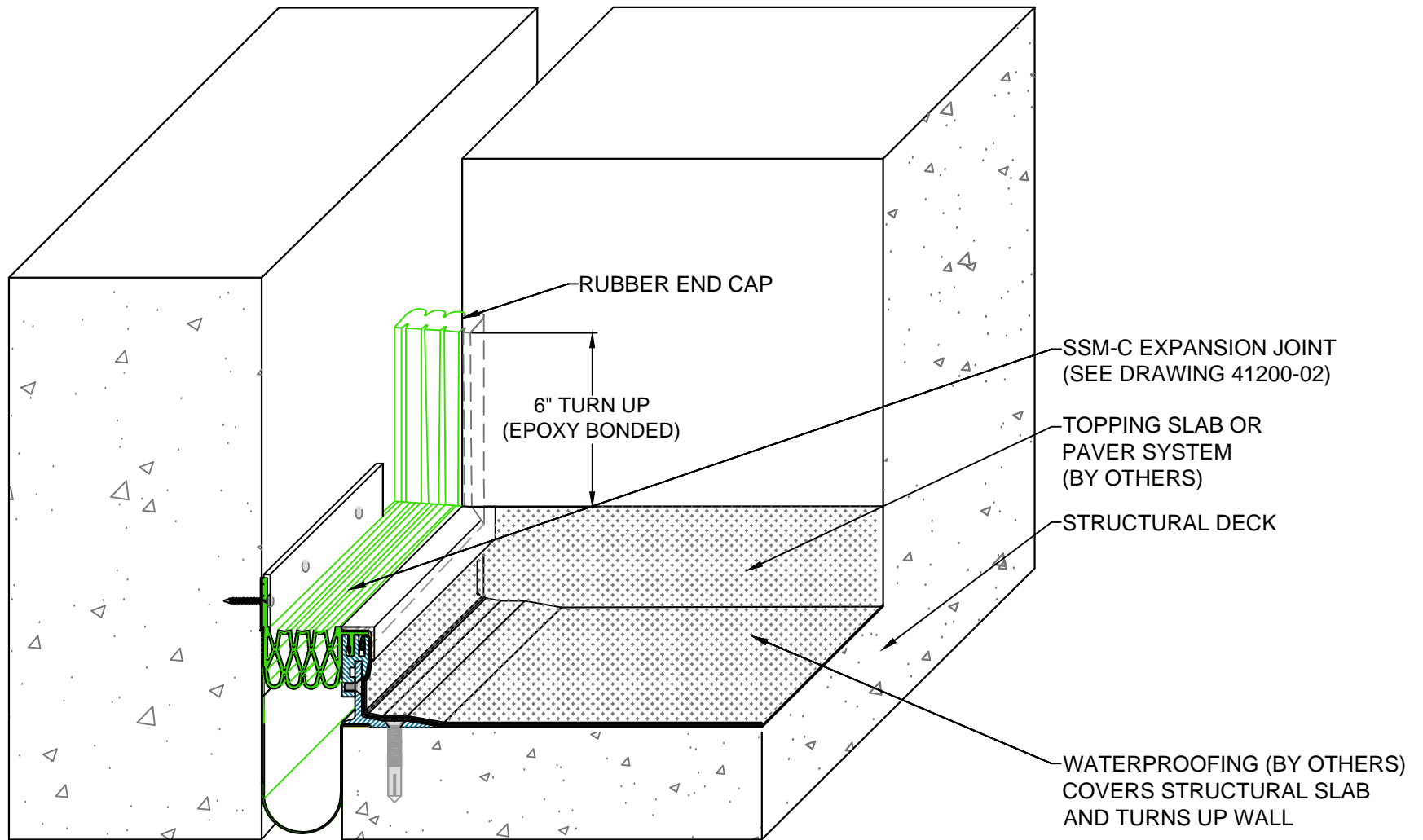
SSM Turn-Up Expansion Joint (Turn-Up Transition)
