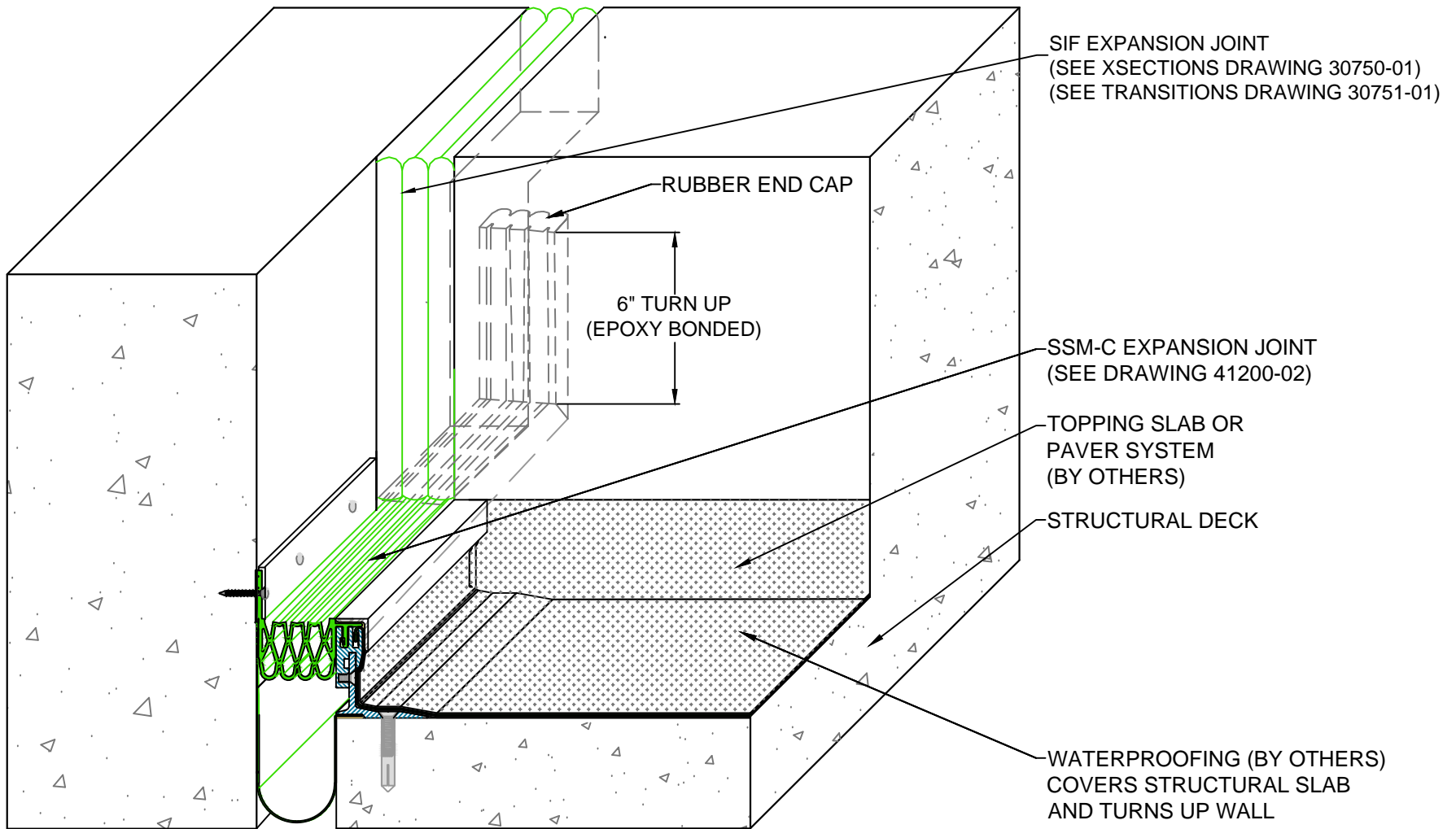
SSM-C-to-SIF Counterflash Expansion Joint (Counterflash Transition)
