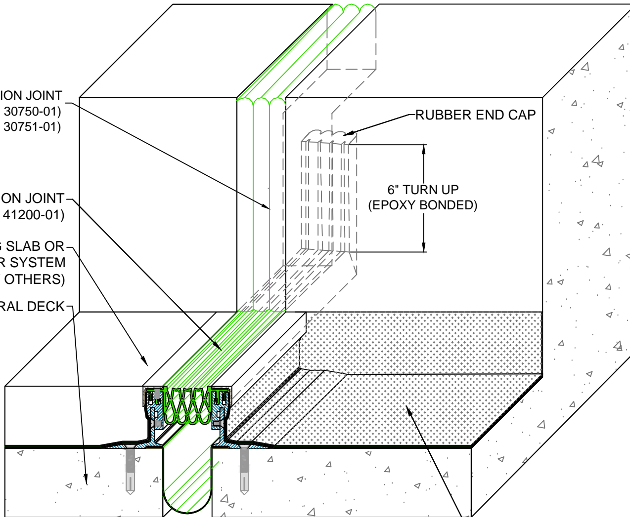
SSM-to-SIF Counterflash Expansion Joint (Counterflash Transition)
