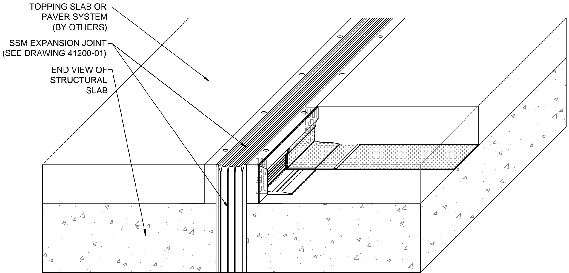
SSM Turn-Down Termination Expansion Joint (End of Slab Turn-Down Termination Transition)
