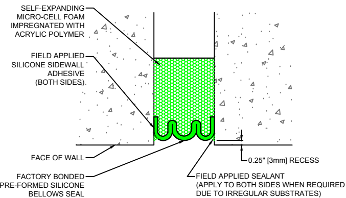
SIF Series Expansion Joint (Wall-to-Wall)
