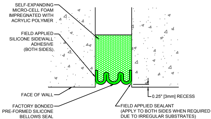
SIF Series Expansion Joint (Wall-to-Wall)
