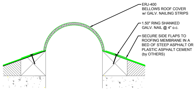
ERJ Series Expansion Joint (Roof-to-Roof)
