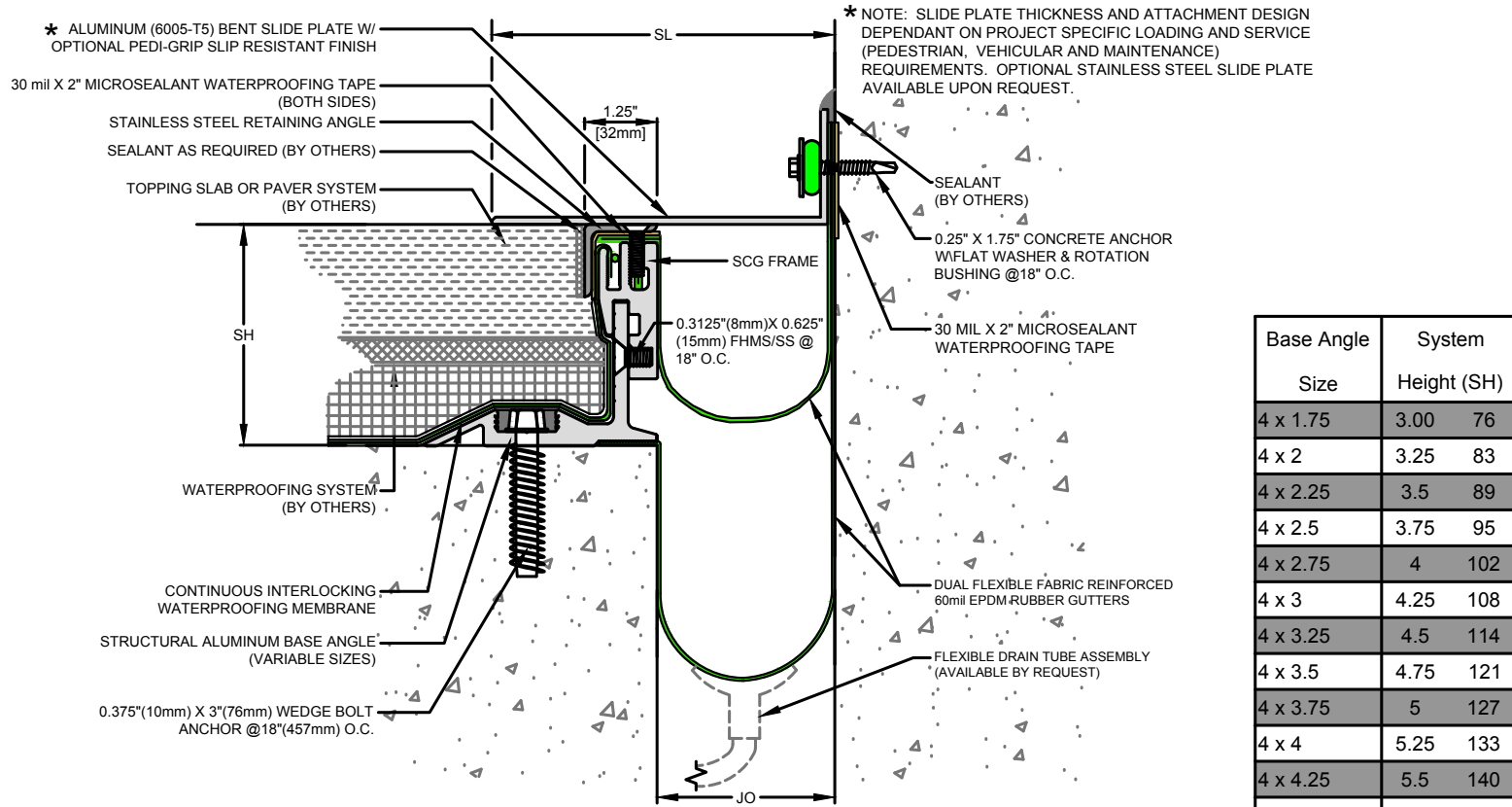
SCG Series Expansion Joint (Slab-to-Wall)
