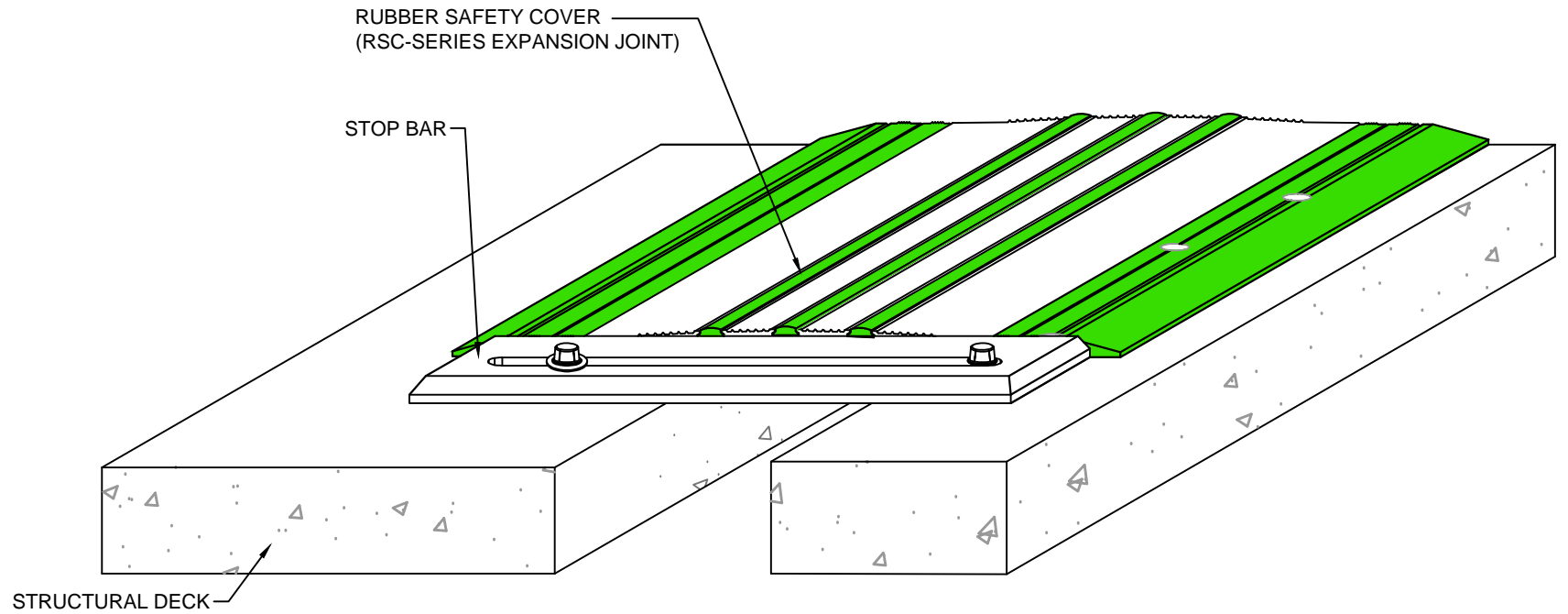
END TERMINATION STOP BAR (USED WHEN THE RSC COVER STOPS BEFORE THE END OF A RUN)
