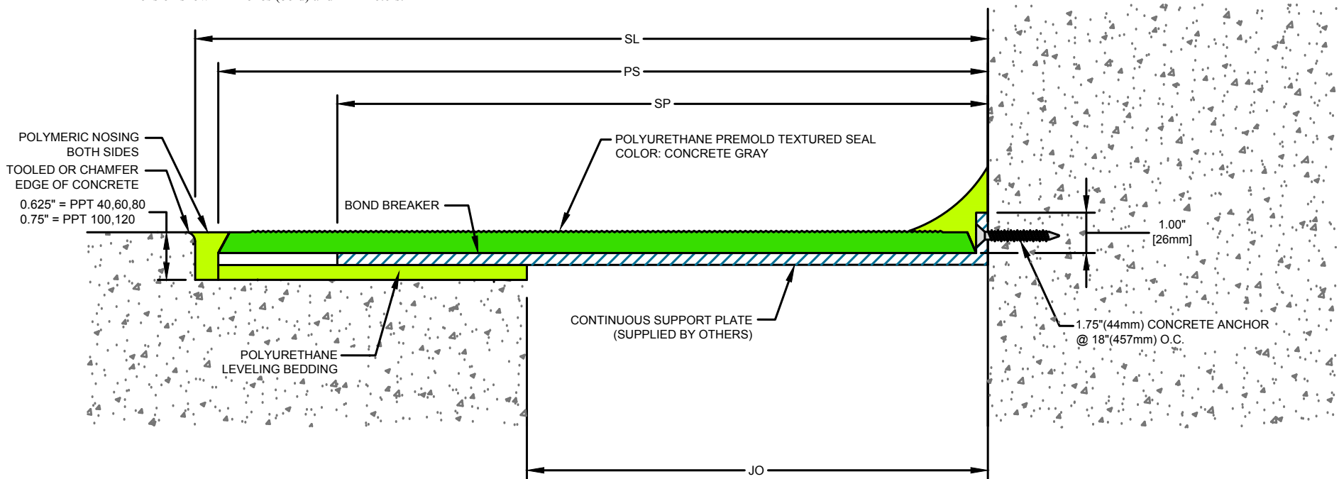
PPT Series Expansion Joint (Slab-to-Wall)
