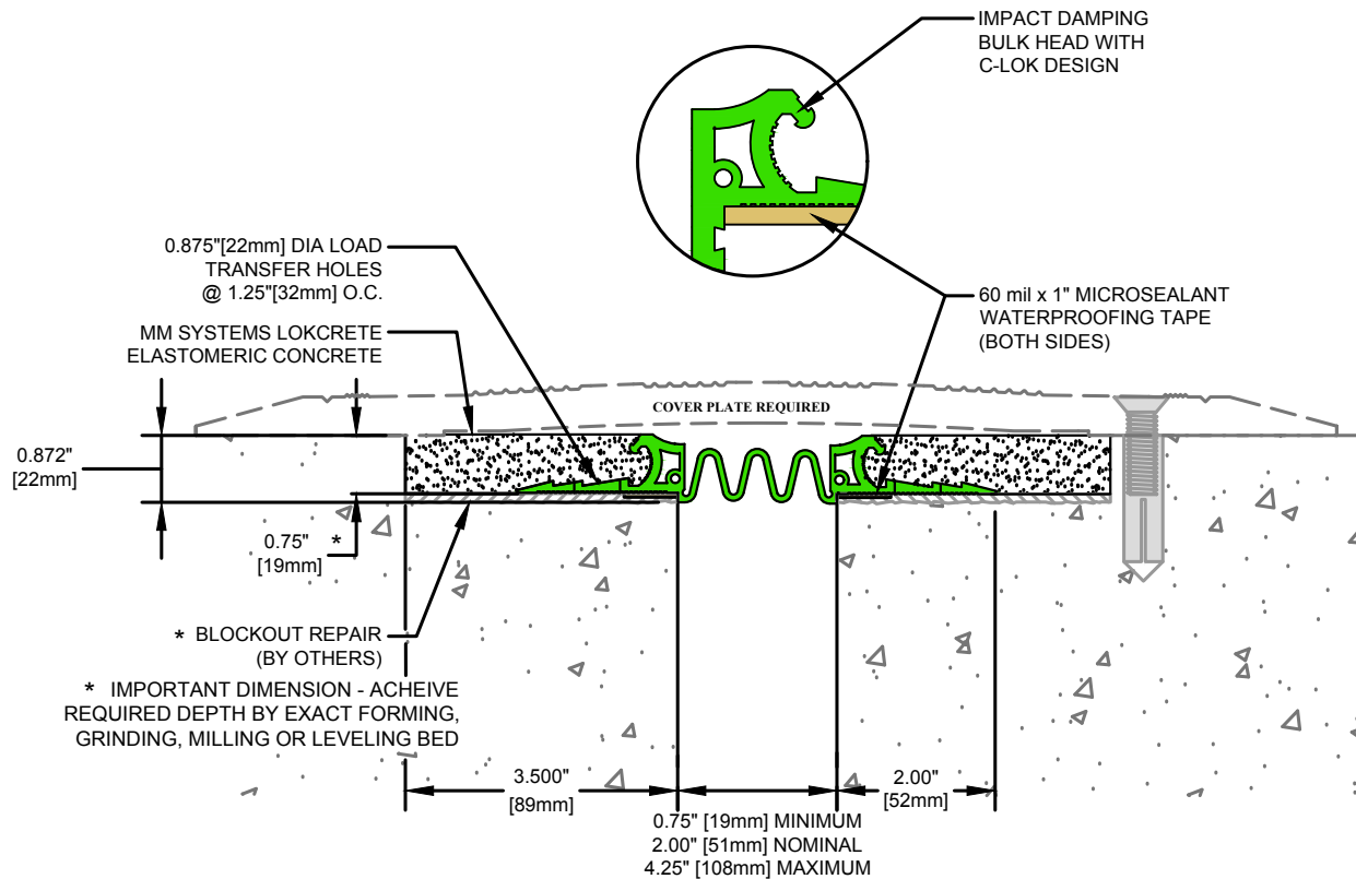
LSS-400 SERIES EXPANSION JOINT (Slab-to-Slab)
