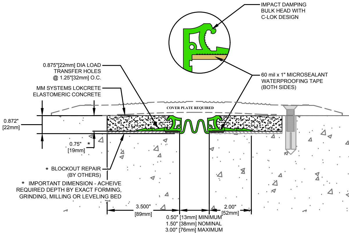
LSS-300 SERIES EXPANSION JOINT (Slab-to-Slab)
