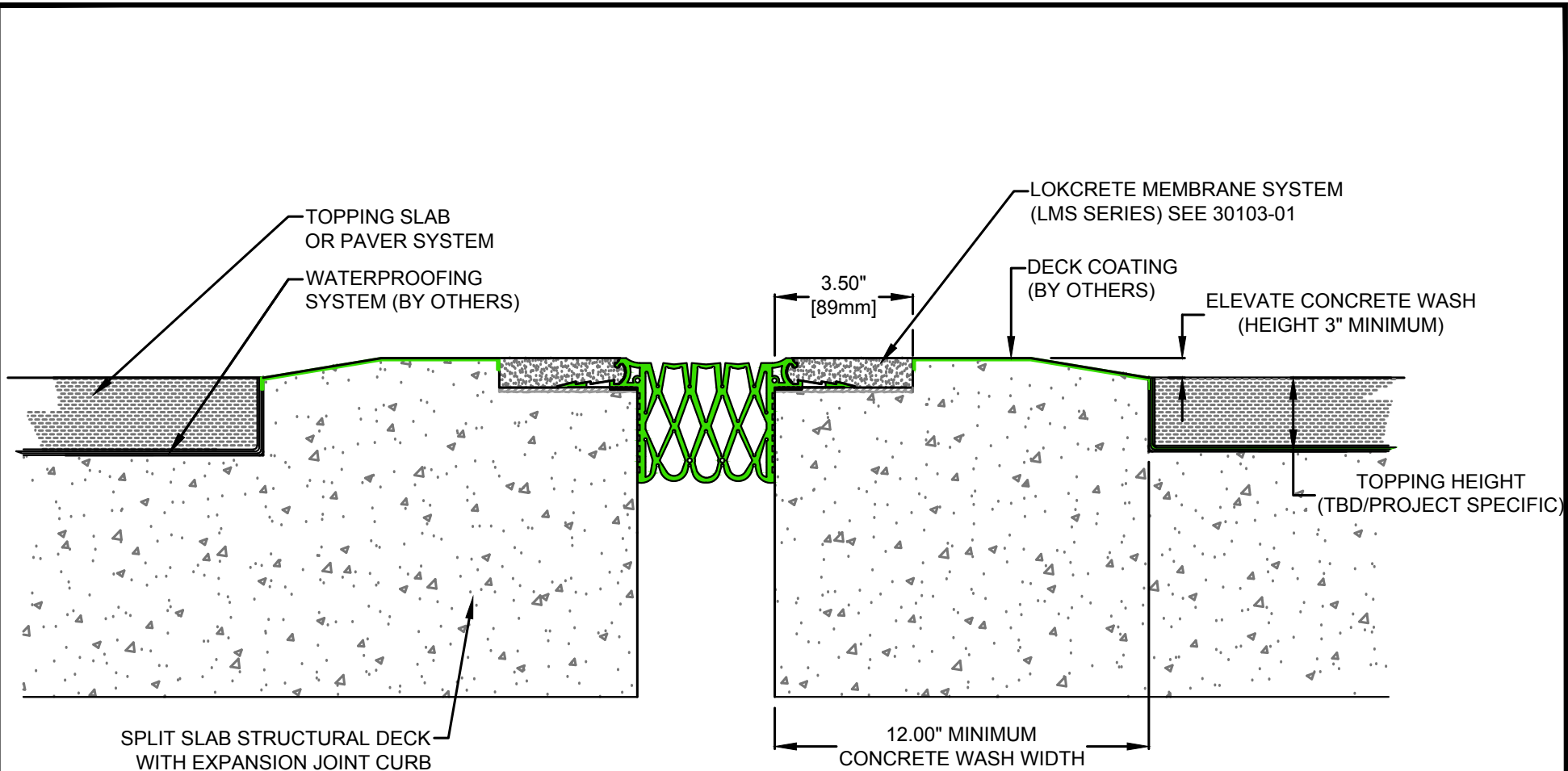
LMS Expansion Joint / Split Slab Construction Detail (Slab-Slab)
