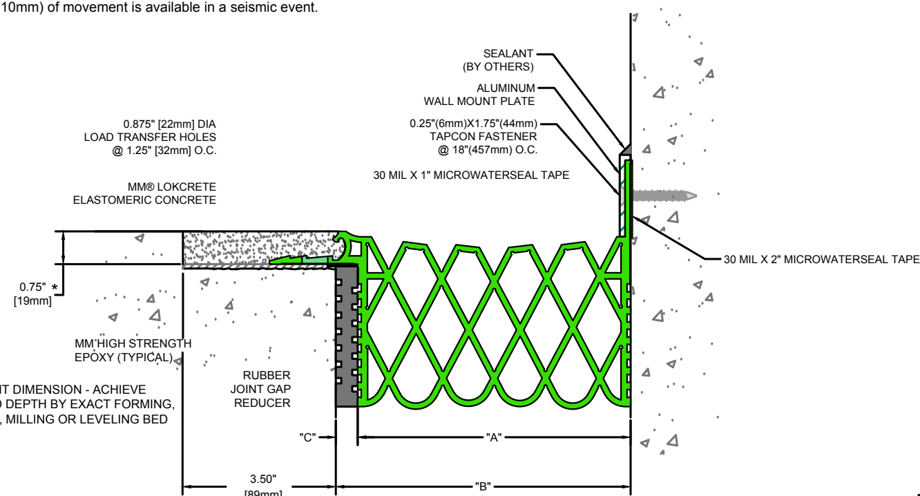
LMS with Joint Gap Reducer (Slab-to-Wall)
