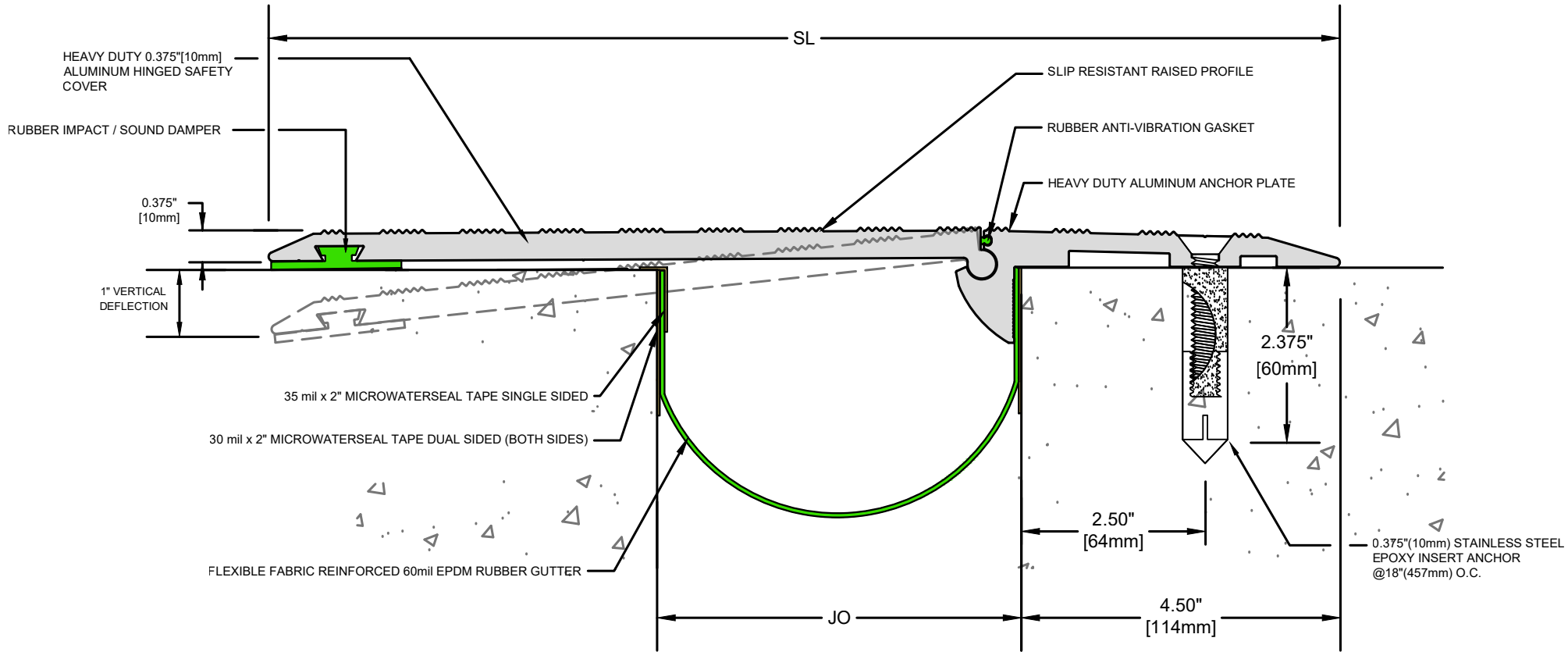
HSC-600 SERIES EXPANSION JOINT (Slab-to-Slab)
