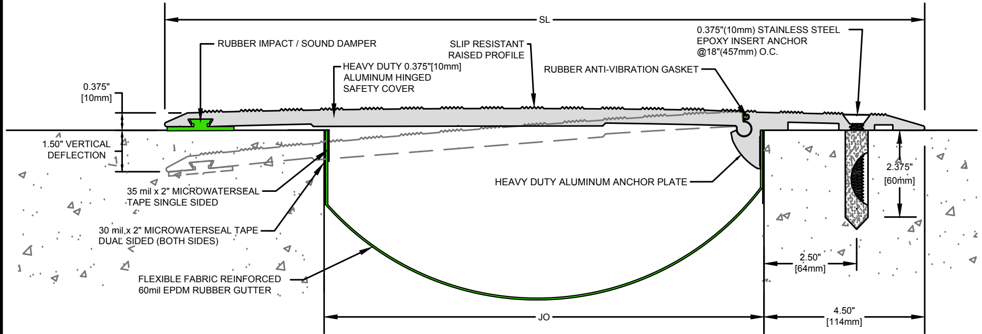
HSC-1000 SERIES EXPANSION JOINT (Slab-to-Slab)
