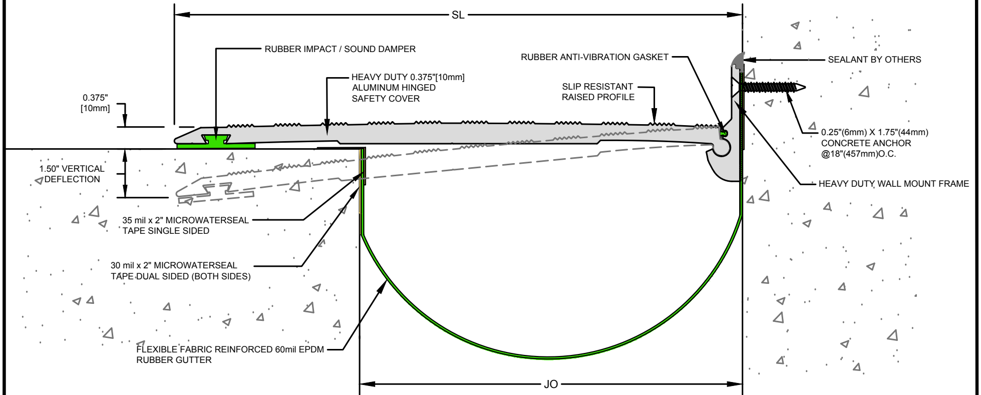
HSC-C-800 SERIES EXPANSION JOINT (SLAB-TO-WALL)
