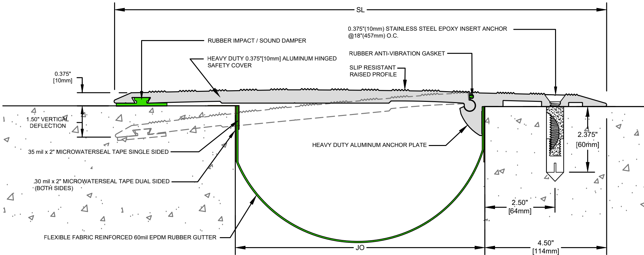
HSC-800 SERIES EXPANSION JOINT (Slab-to-Slab)
