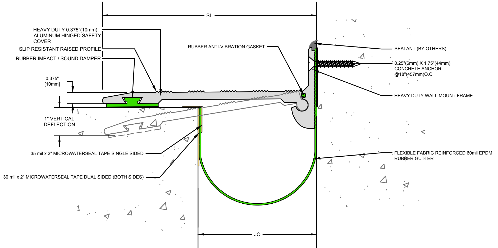
HSC-C-400 SERIES EXPANSION JOINT (Slab-to-Wall)
