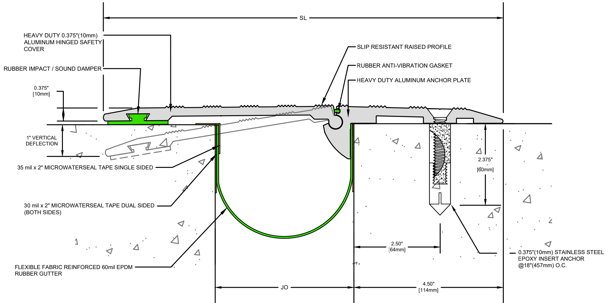
HSC-400 SERIES EXPANSION JOINT (Slab-to-Slab)
