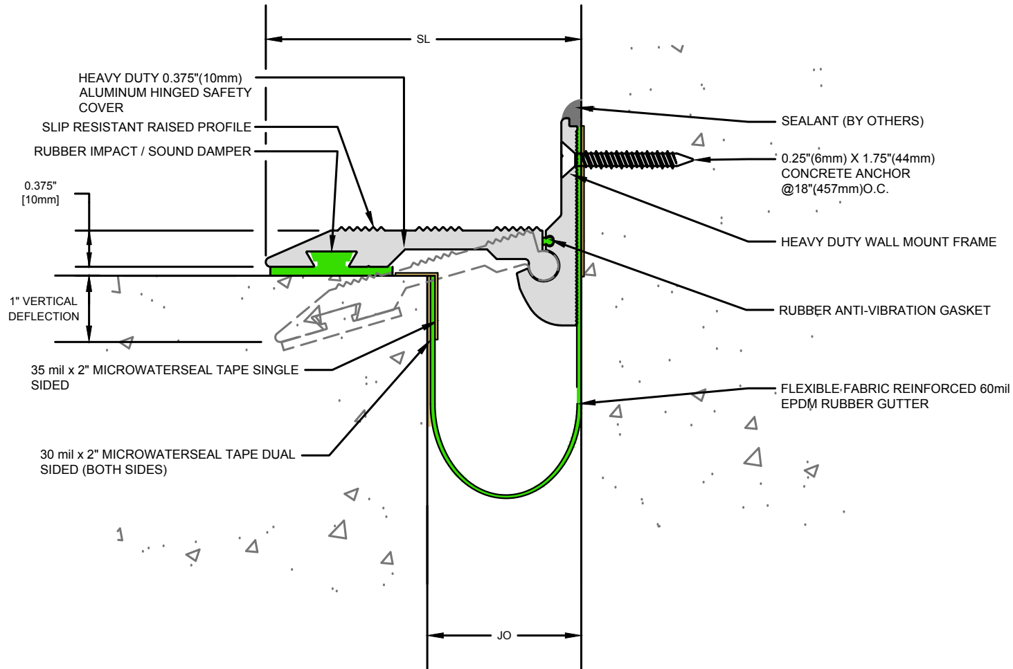
HSC-C-200 SERIES EXPANSION JOINT (Slab-to-Wall)
