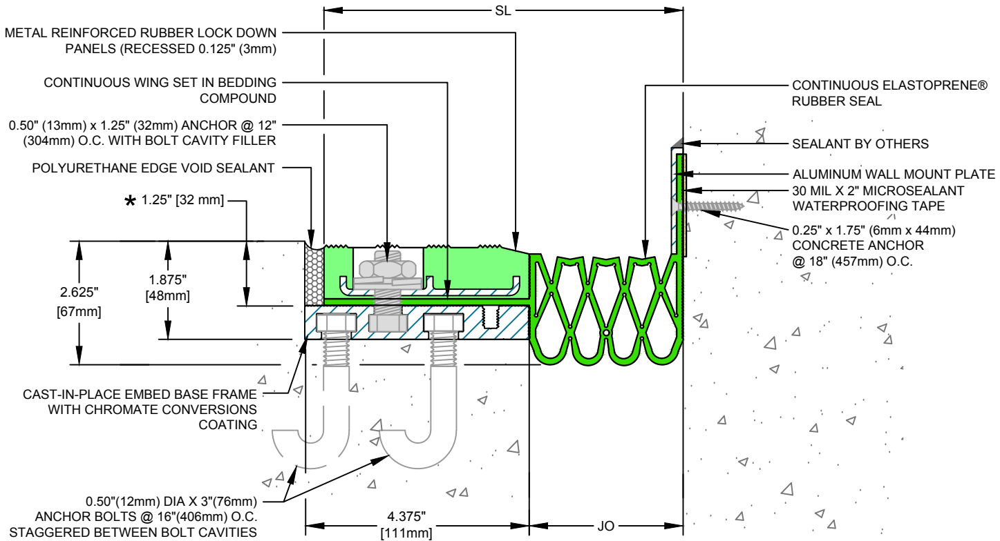
EMC Series Expansion Joint (Slab-to-Wall)
