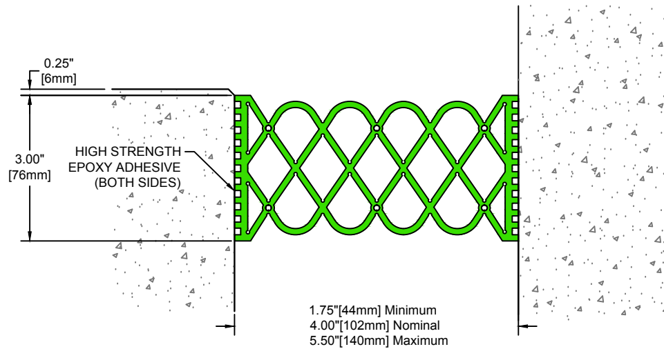
Slab-to-Wall
