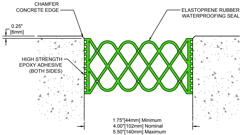
Slab-to-Slab
