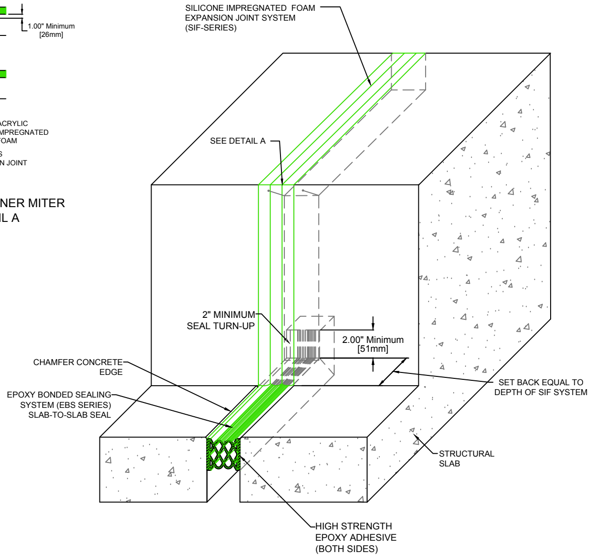
EBS-to-SIF Counterflash Expansion Joint Transition (Slab-to-Slab)
