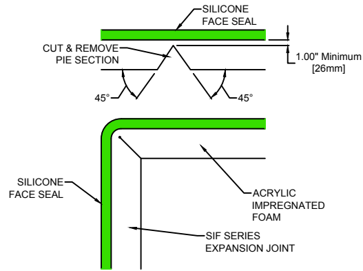
OUTSIDE CORNER MITER DETAIL A
