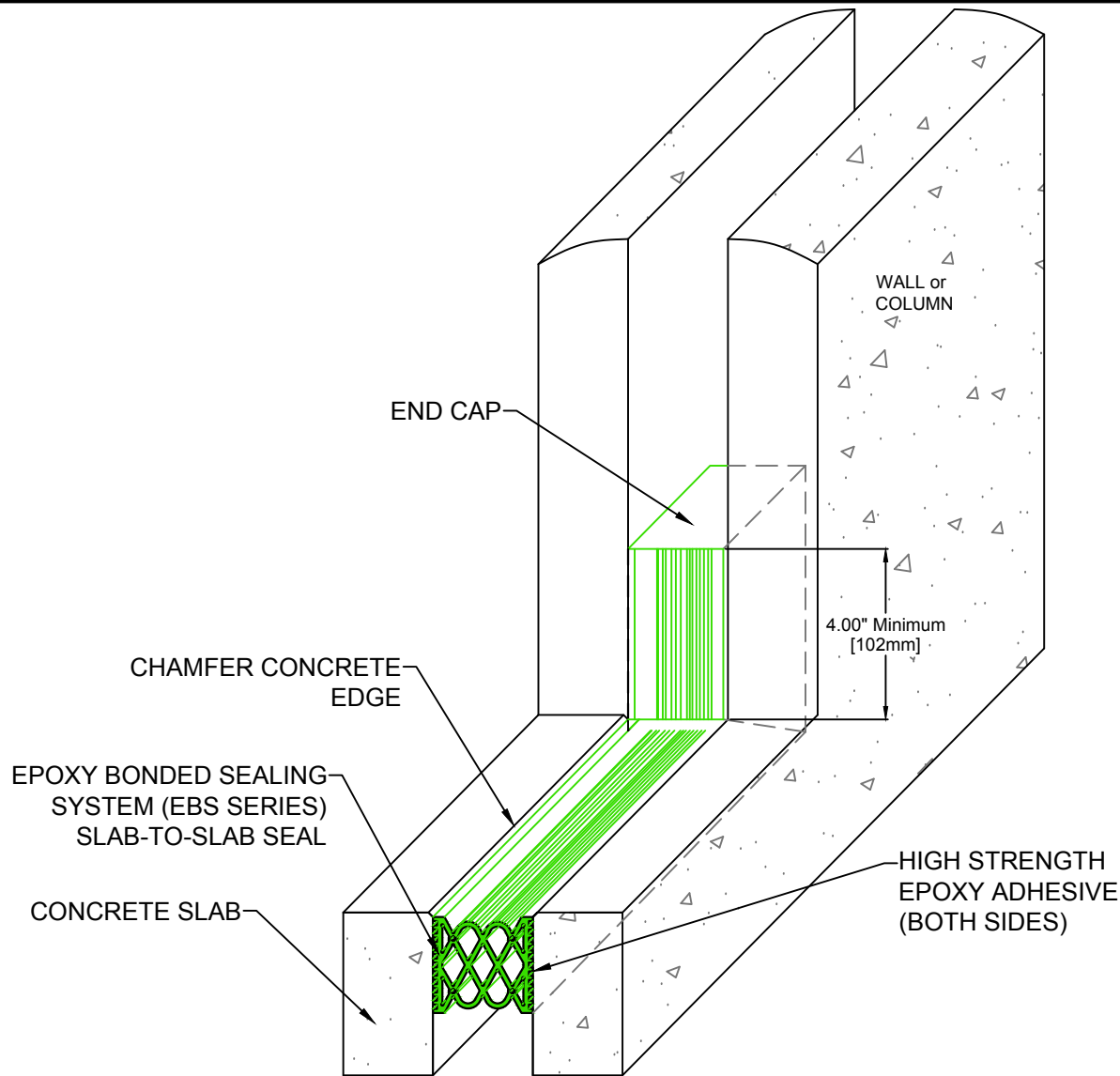
EBS Turn Up Expansion Joint Transition (Slab-to-Slab)
