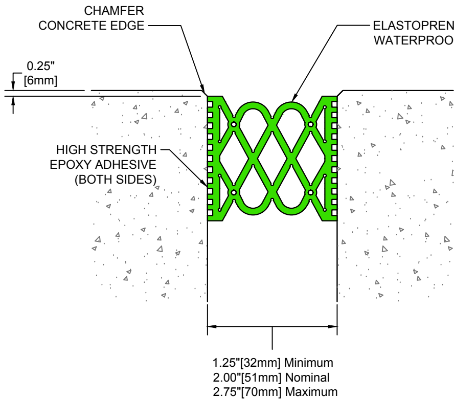
Slab-to-Slab
