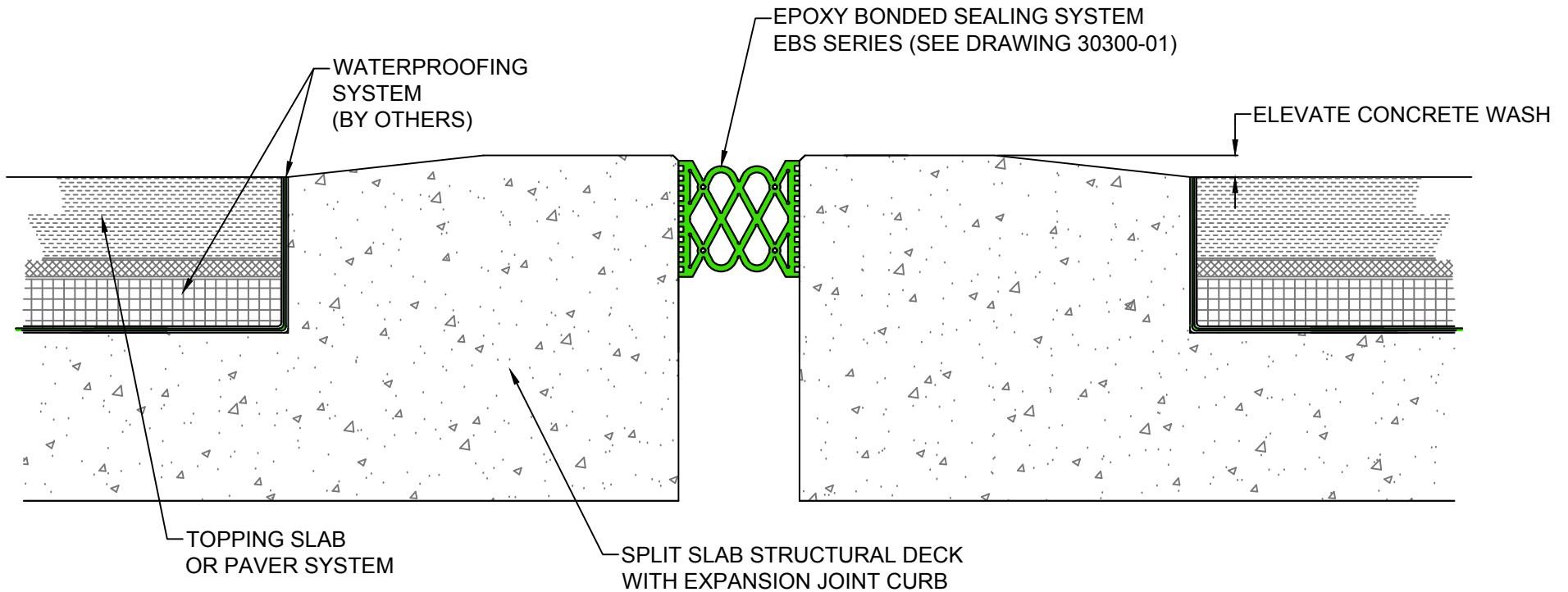
EBS Expansion Joint (Slab-to-Slab / Concrete Wash - Split Slab)
