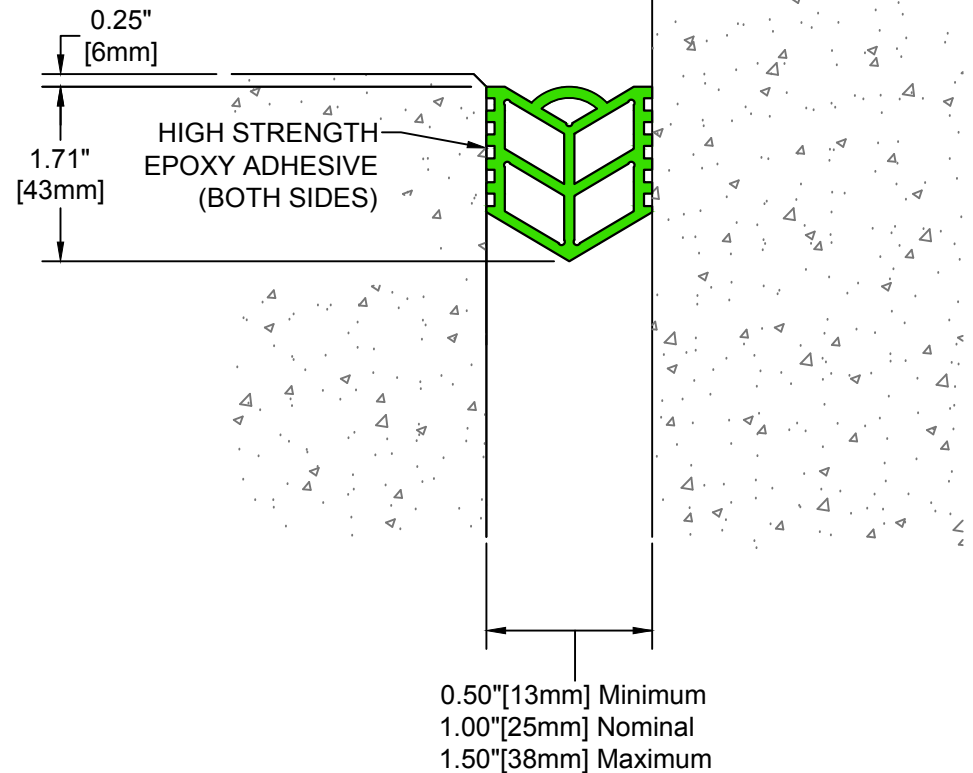
Slab-to-Wall
