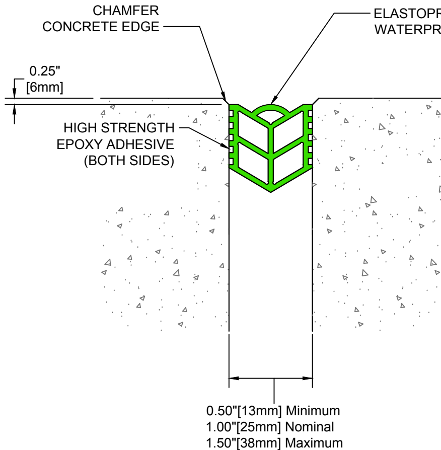
Slab-to-Slab
