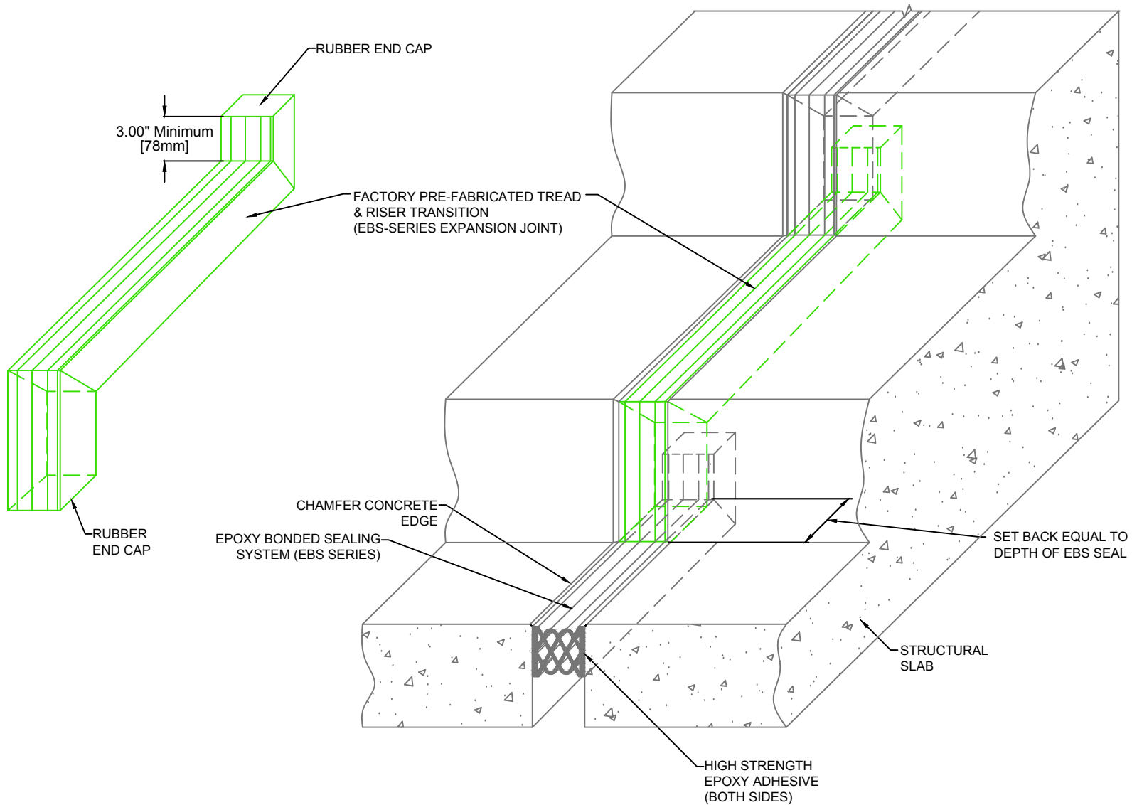
EBS Tread & Riser Expansion Joint Transition (Slab-to-Slab)
