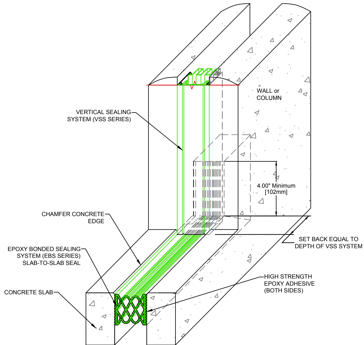
EBS-to-VSS Expansion joint Transition (Slab-to-Slab)
