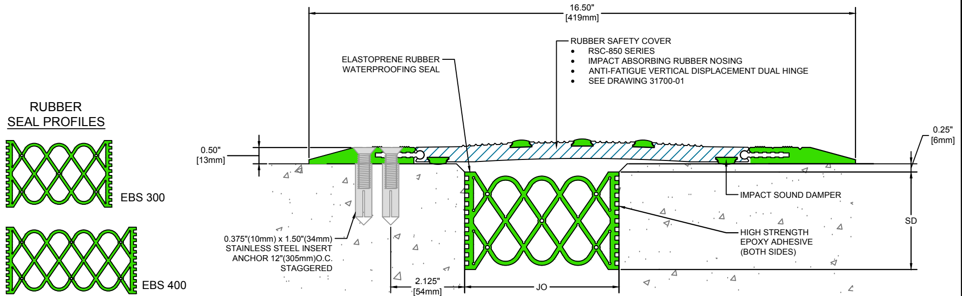
EBS with RSC-850 Expansion Joint Cover (Slab-to-Slab)
