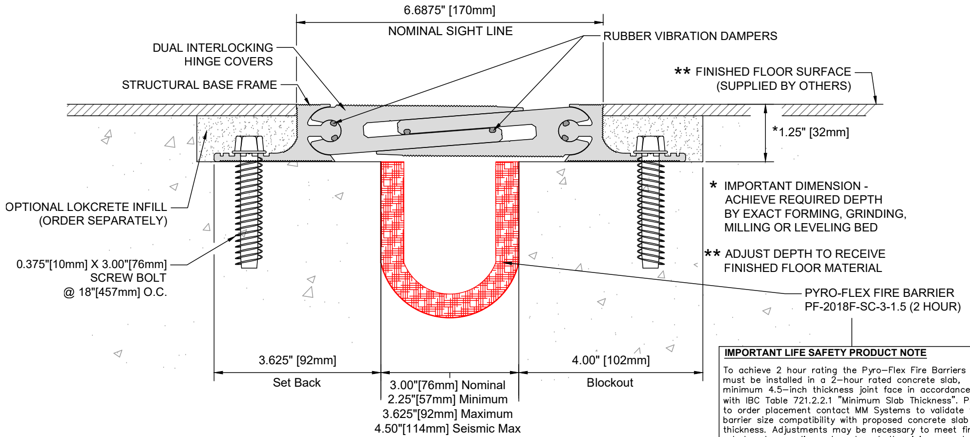
DIH-300 Fire Rated Expansion Joint (Floor-to-Floor)
