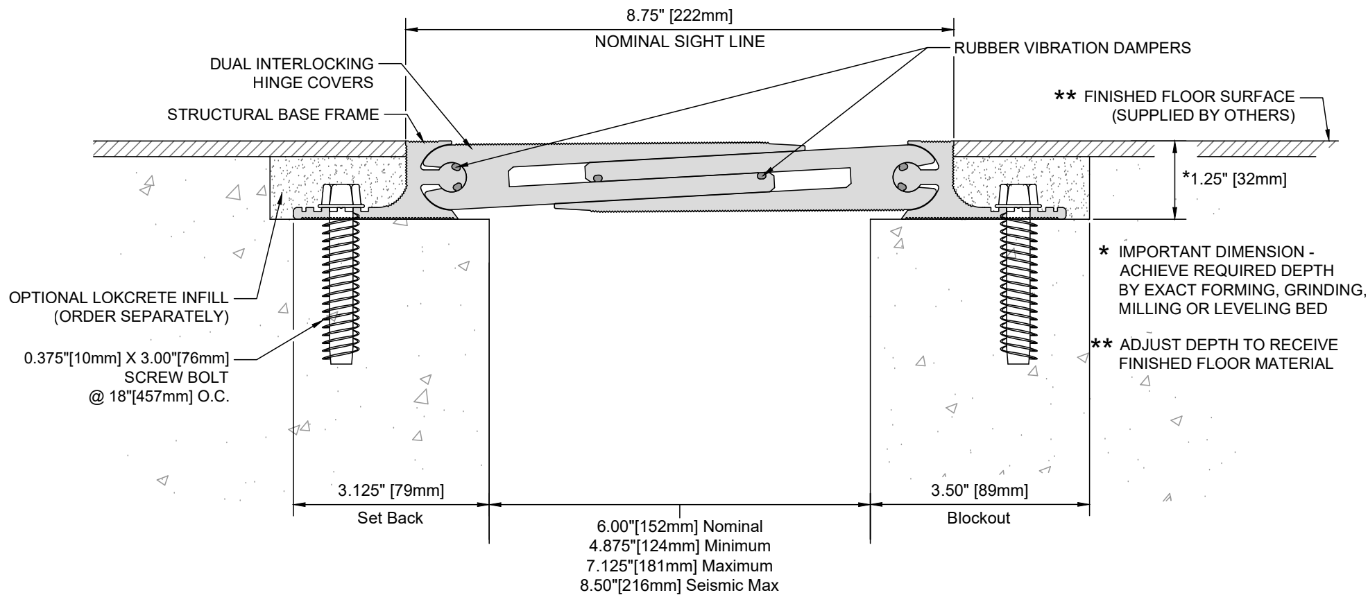
DIH-600 Series Expansion Joint (Floor-to-Floor)
